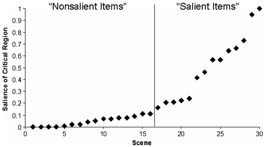
Figure 2. Mean saliency value of pixels within the critical region within each of the 30 scenes. Sixteen scenes were considered to have nonsalient critical regions; fourteen scenes were considered to have salient critical regions.
